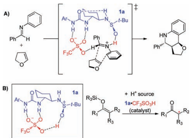
Figure 1. (A) Schematic representation of the geometry and energy-minimized lowest energy transition structure for sulfinamide–urea/TfOH cocatalyzed Povarov reaction (from ref 5). (B) Schematic representation of the energy-minimized lowest energy ground state structure for the sulfinamide–urea 1a /TfOH ‘chiral acid’ complex. Structures calculated at the B3LYP/6-31G(d) level of density functional theory. Ar = 3,5-bis(CF 3 )C 6 H 3 .
